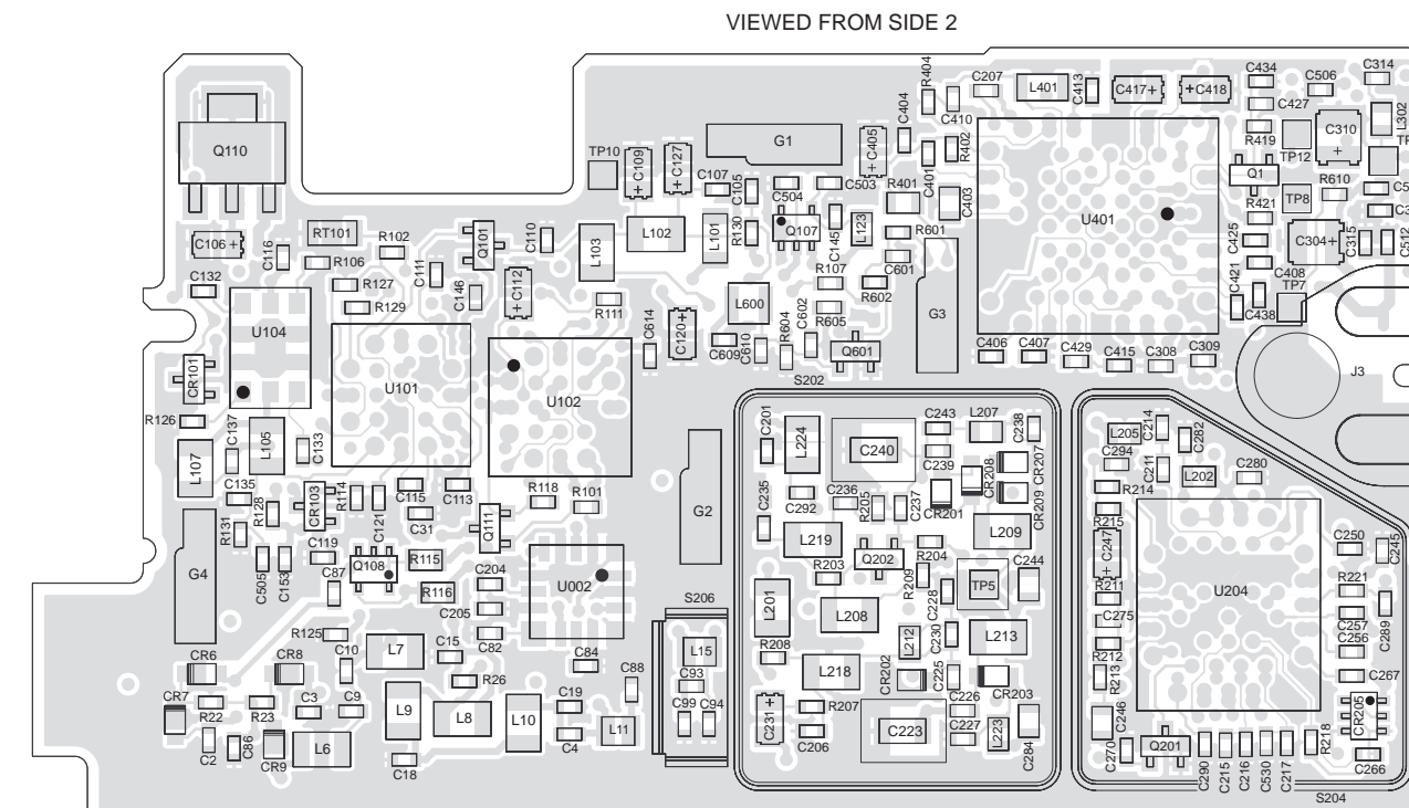
NLE4244P UHF Range 2 Transceiver Circuit Board Details and Parts List
